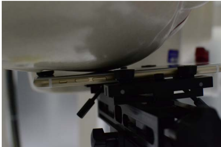
Figure 2: Head Right side View with Cell Shield with DASY Test System
