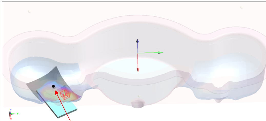
Figure 3.2-6 CAD Model of Head view with Cell Shield placed on iPhone 6
