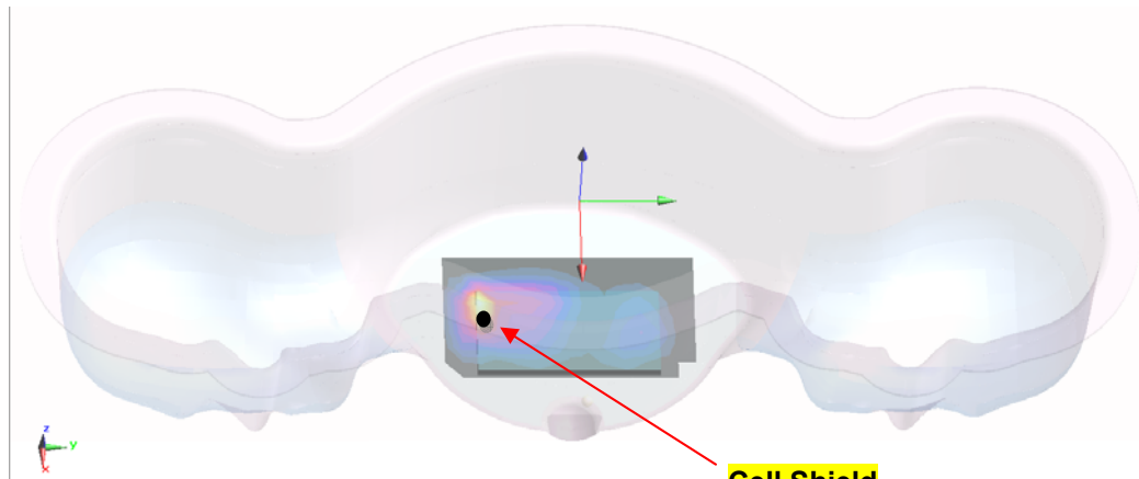
Figure 3.2-3 CAD Model of body back side view with Cell Shield placed on Iphone 6
